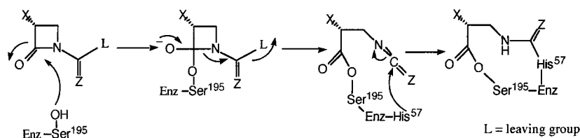
Scheme 1. Potential suicide mechanism of elastase inhibition
