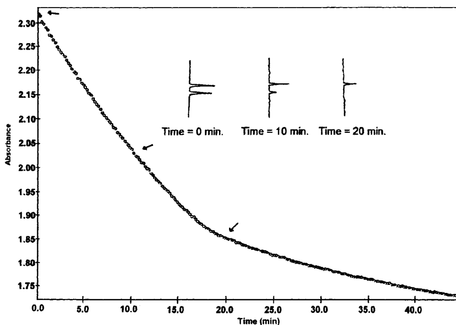
Figure 1. Elastase-catalyzed hydrolysis of 6c ; the absorbance of a 2 \cdot 10^{-4} \text{ M} solution of 6c was monitored in the presence of 1.9 \cdot 10^{-6} \text{ M} PPE at 232 \text{ nm} \text{pH} = 7.67 ; inset: GC analysis on a Chrompack chiral-dex capillary column of the mixture during hydrolysis
