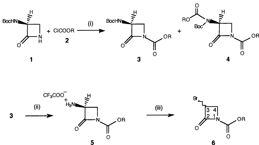
Scheme 2. Preparation of 1-alkoxycarbonyl-3-bromoazetidion-2-ones; reactions conditions: (i) LiHMDS, THF, -78°C, 30 min, then 2 , -78°C to 20°C, 1 h; 3a : R = CH 2 Ph, yield 89%, 3b : R = CH 2 CCl 3 , yield 69%, 3c : R = CH 2 CF 3 , yield 83%; (ii) CF 3 COOH, 20°C, 30 min; (iii) KBr, 2.5 N H 2 SO 4 /EtOH, NaNO 2 , 6–8°C, 3 h; 6a : R = CH 2 Ph, yield 80%, 6b : R = CH 2 CCl 3 , yield 23%, 6c : R = CH 2 CF 3 , yield 56%
