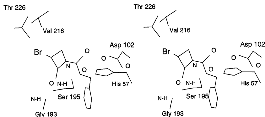
Figure 2. Stereodiagram representation of the docking of 6a in the active site of PPE
