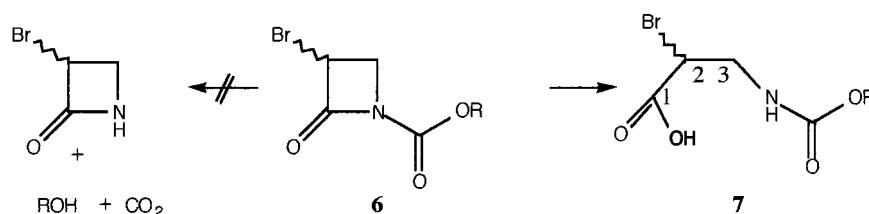
Scheme 3. Hydrolysis product of 1-alkoxy-carbonyl-3-bromoazetid-2-ones
